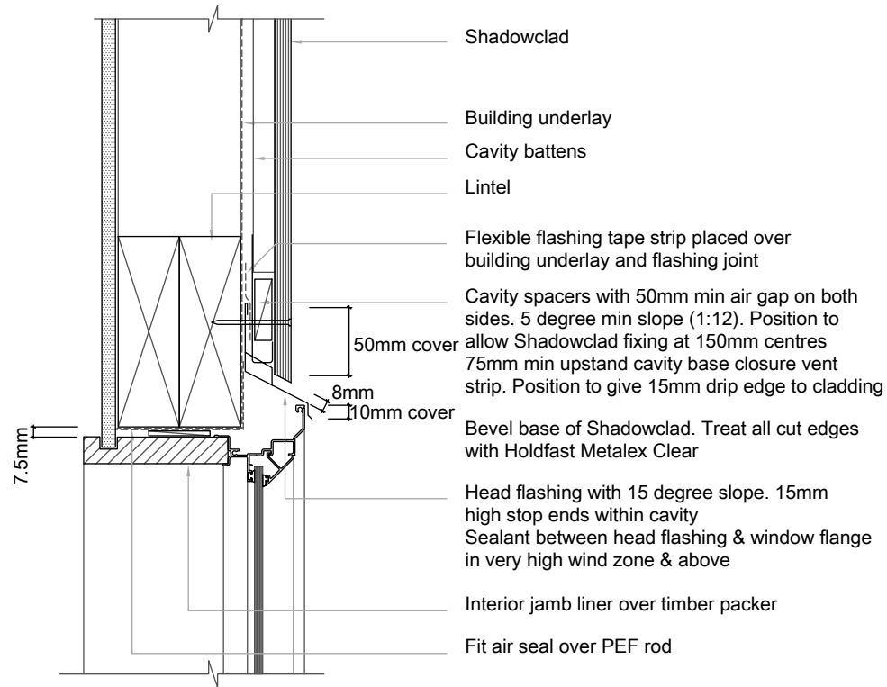
SC028 Shadowclad Window Head (Cavity)
