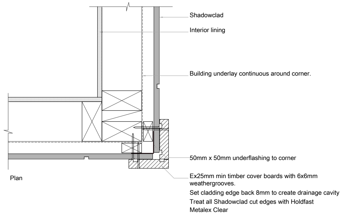
SC022 Shadowclad External Corner w/ Cover Boards (Cavity)
