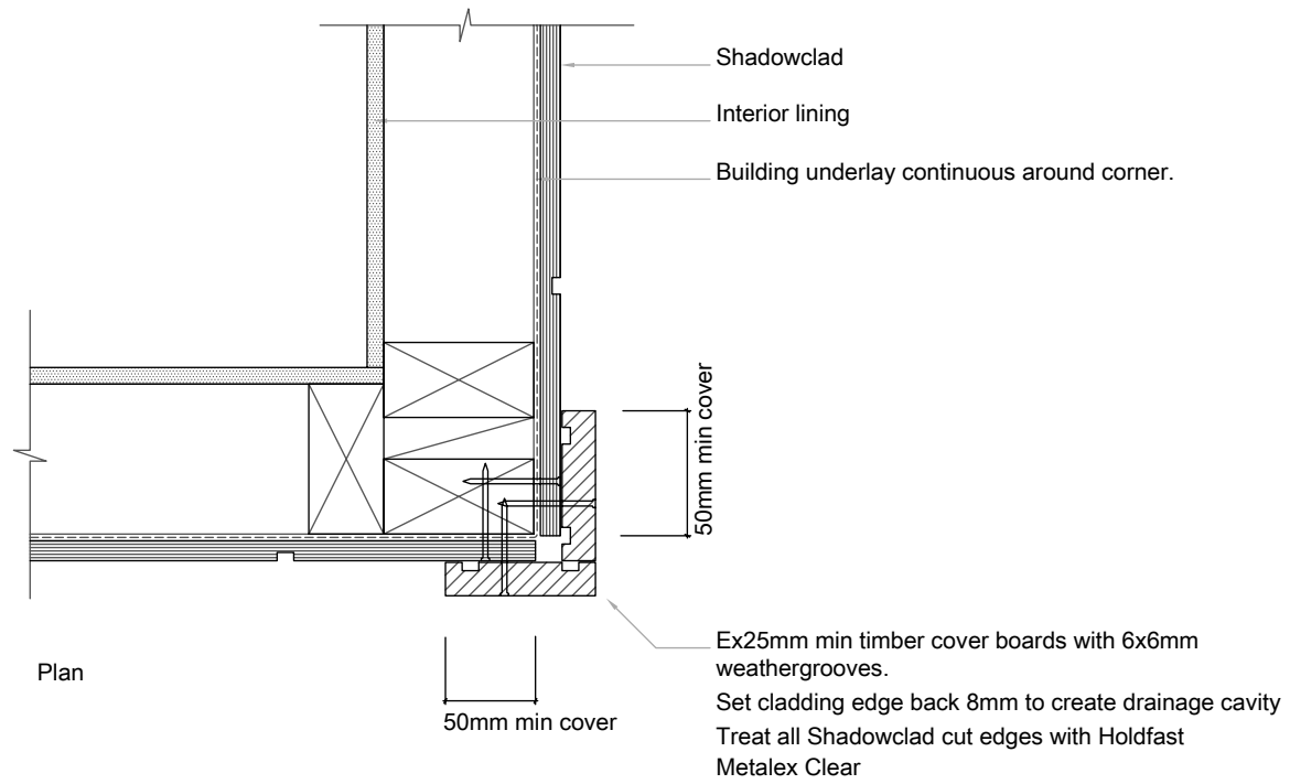
SC021 Shadowclad External Corner w/ Cover Boards (Direct)
