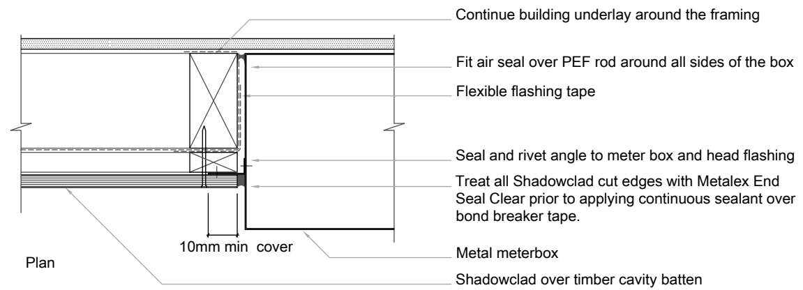
SC034B Shadowclad Meterbox Top Profile (Cavity)
